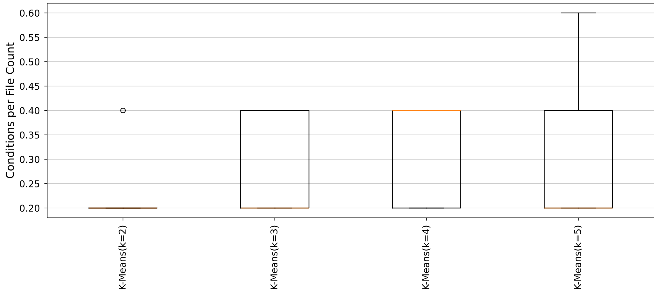
YARA Rules Conditions per File Count Distribution (Cluster44_Size5 dataset)
